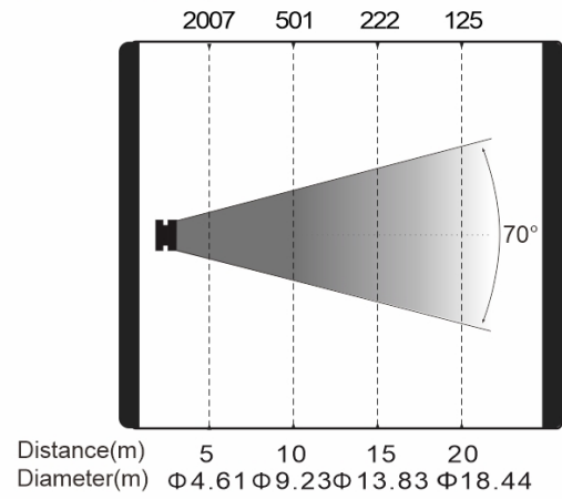
Intensity LUX (70°)
