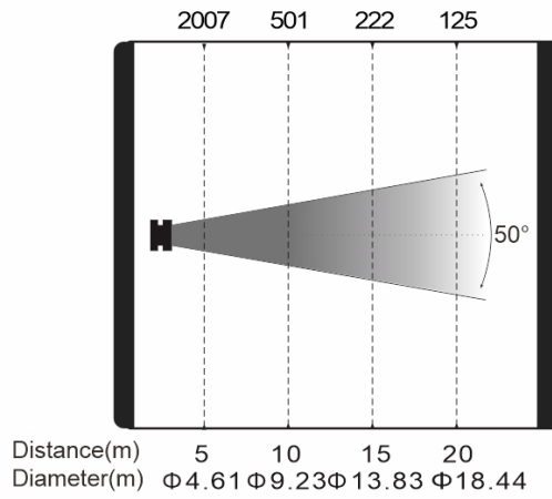
Intensity LUX (50°)
